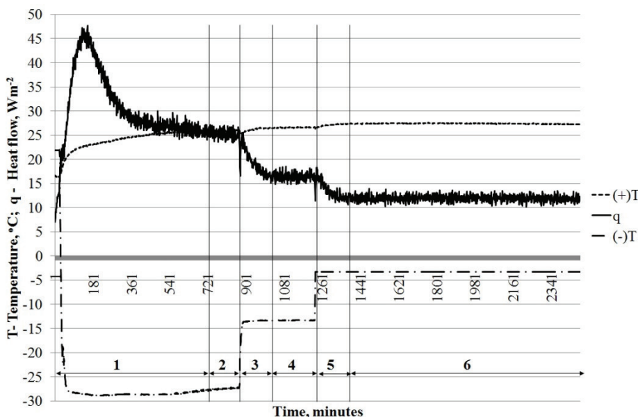
Figure 3. Maple leaf sample, thickness 165 mm. Value of heat flux depending on differences of temperatures. Horizontal axis: Time – minutes, sampling rate – 1 sample each minute. Vertical axis: (+)T – positive room temperature, ^\circ\text{C} ; (-)T – negative chamber temperature, ^\circ\text{C} ; q – heat flux, \text{W m}^{-2} (only positive values). Temperature and heat flux values have the same scale. 1, 2, 3, 4, 5, 6 – time periods of change and stability for temperature and heat flux.
